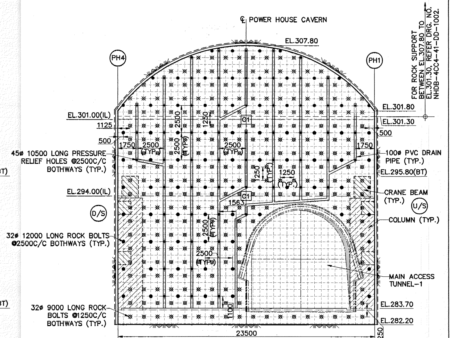
TYPICAL CROSS SECTION-END WALL SERVICE BAY-1 (MAT-1 SIDE) A
